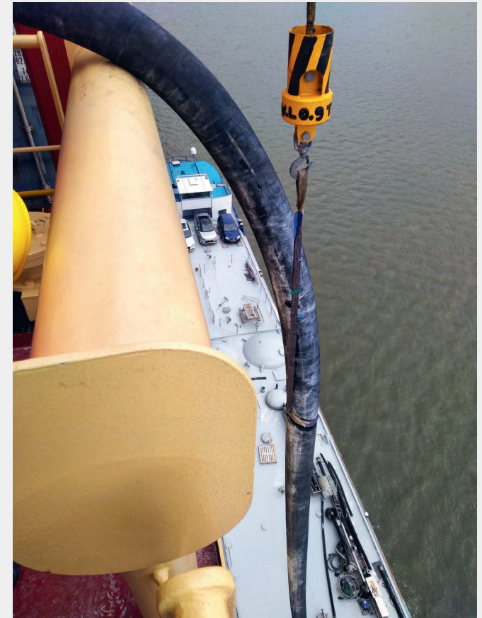
Example of MagTreat® being supplied to a ship from a barge equipped with a pump. Pumping the product onboard using a hose
